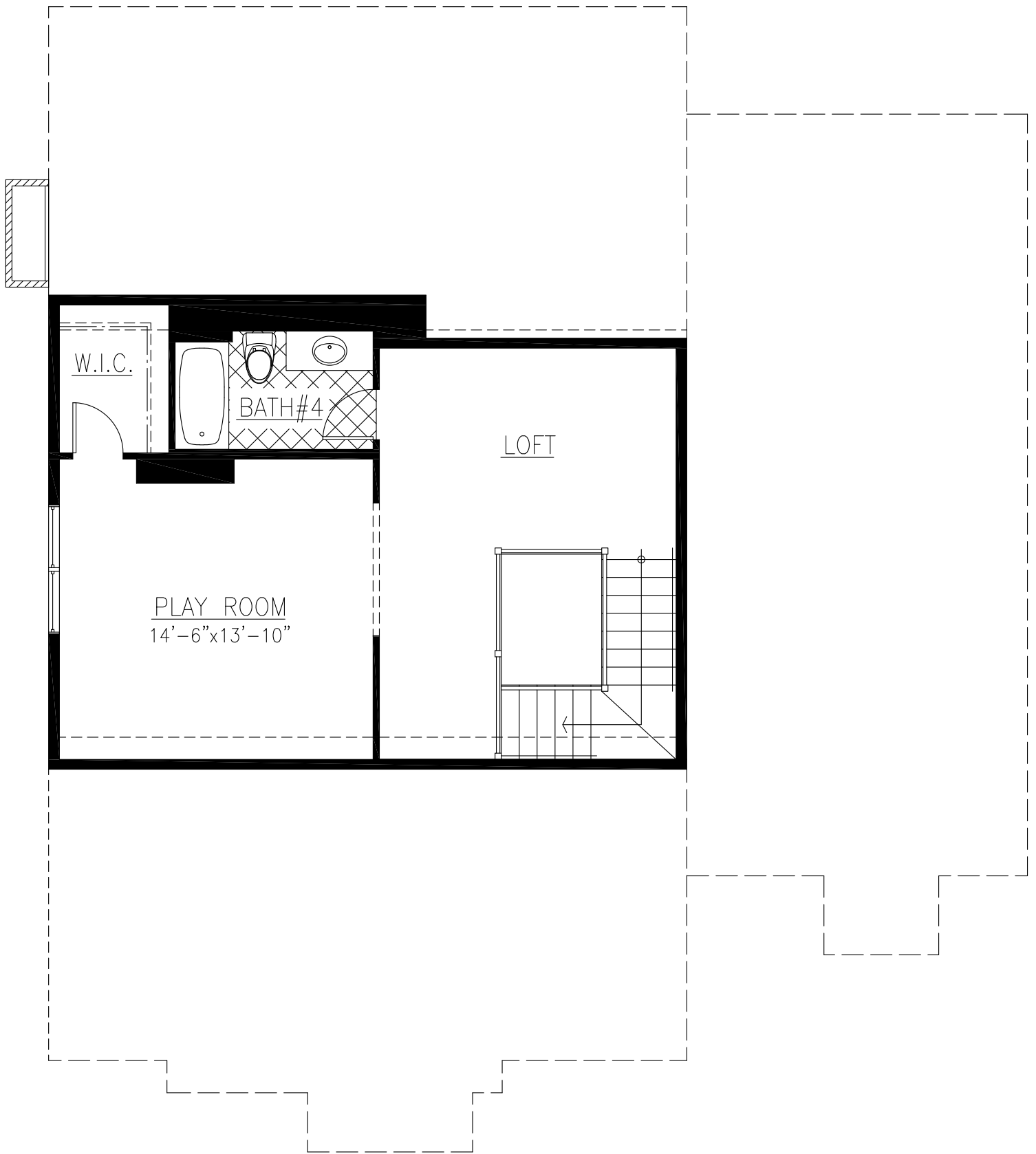
Attic Level Plan Drawing
