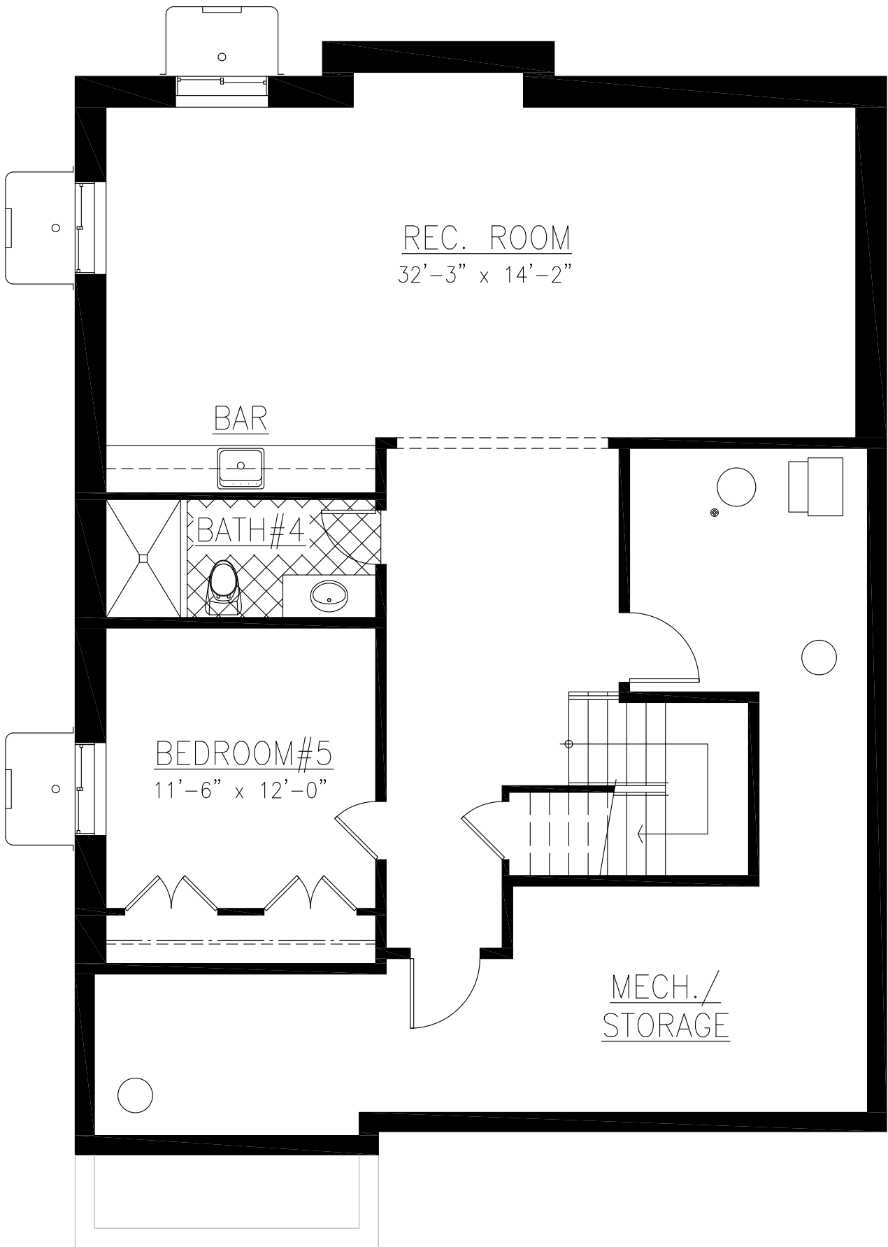
Finished Basement Plan Drawing
