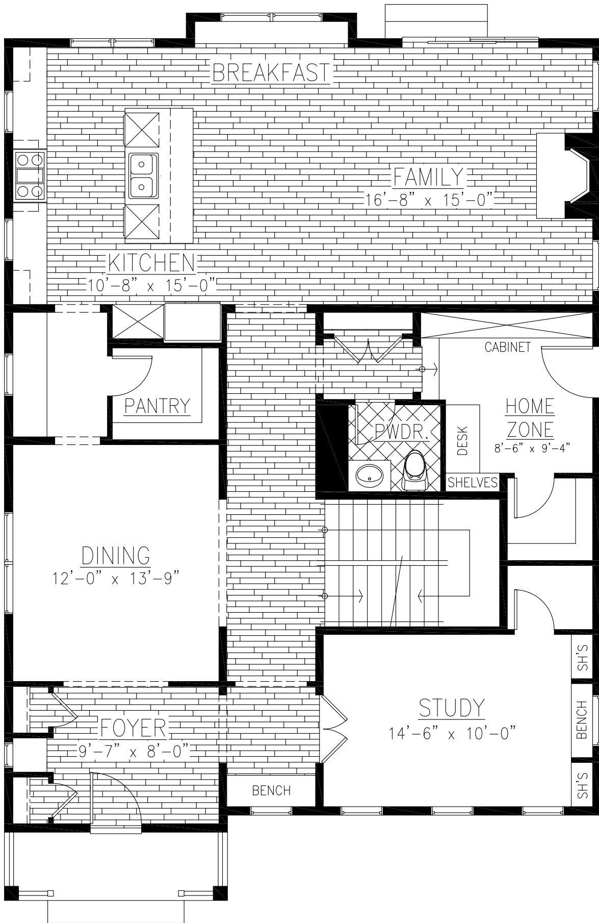
First Floor Plan Drawing
